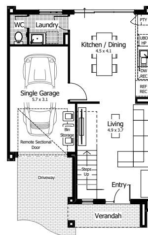
Ground Floor Layout 1:100
