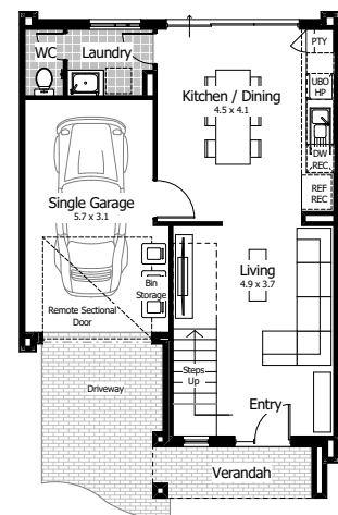
Ground Floor Layout 1:100
