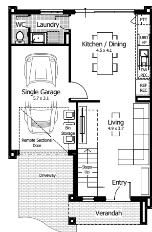
Ground Floor Layout 1:100
