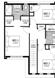
DESIGN FIRST FLOOR 1:100
