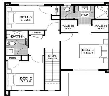
DESIGN FIRST FLOOR 1:100
