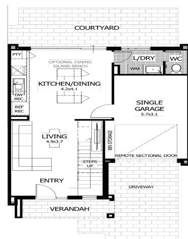
DESIGN GROUND FLOOR 1:100
