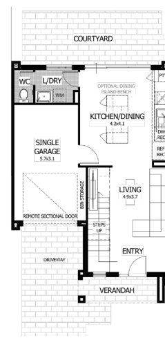
DESIGN GROUND FLOOR 1:100
