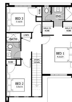
DESIGN FIRST FLOOR 1:100
