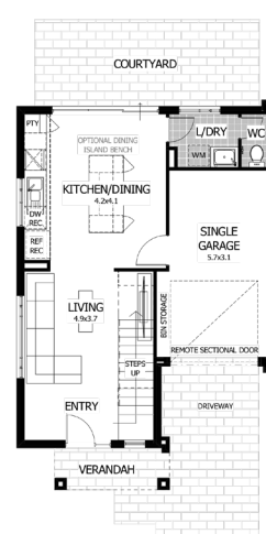
DESIGN GROUND FLOOR 1:100
