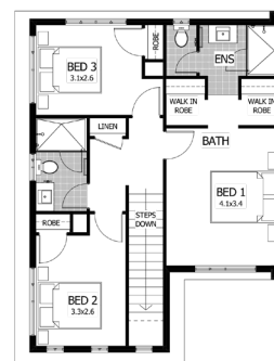
DESIGN FIRST FLOOR 1:100
